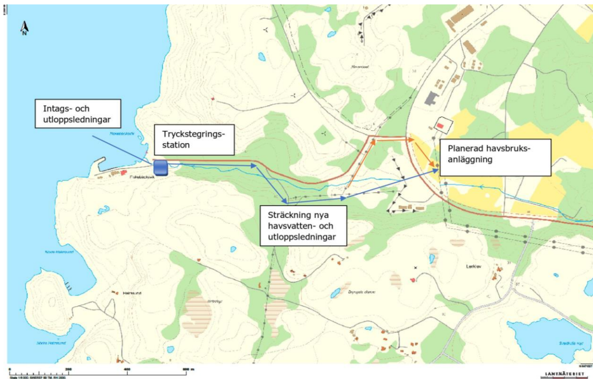
Figure 4. Overview of the proposed pipeline route for the inlet and outlet pipes to the industrial park.
